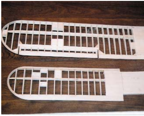
Above: The wing structures have sheet covering and various balsa blocks that will support struts, rigging-wire fittings, and dummy running lights.
