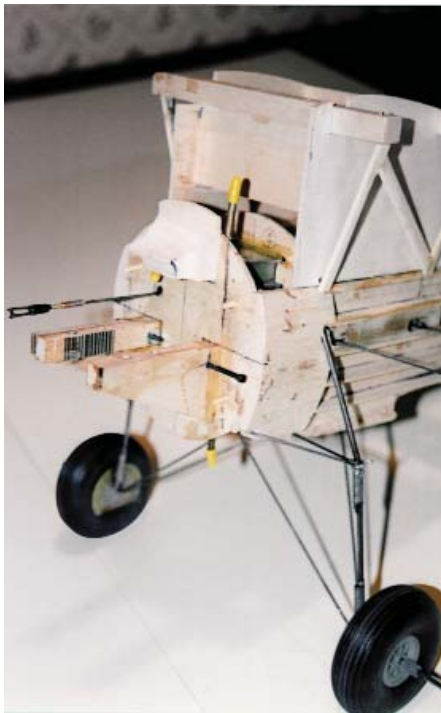
Left: A simple fixture is used to accurately install and align the cabane struts. The undercarriage wire loops at the strut juncture, which will anchor the dummy rigging wire.
