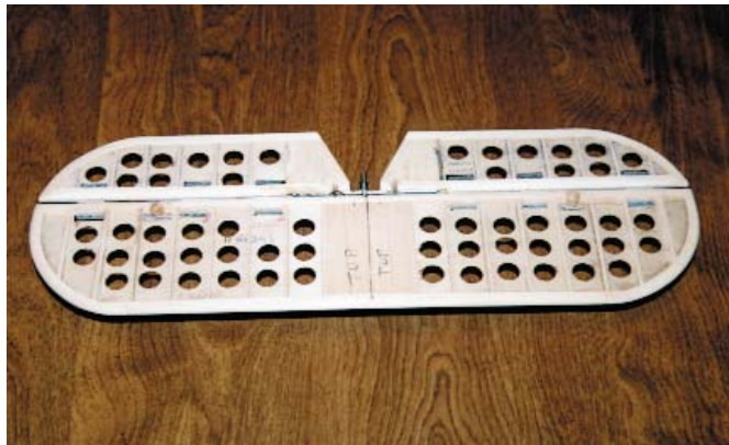
The horizontal tail surfaces require weight-saving holes in the 1/64 plywood core. A Forstner bit is the best tool for making those holes.
