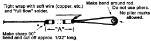
Figure 1A. Two Line Construction For Use With Button-Type Bellcranks. "Double Loop" Termination.
