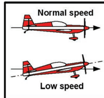
Fig. 3 At normal speed, the attitude is similar to the flight path. When the speed is reduced, the attitude may change to maintain a constant flight path.
