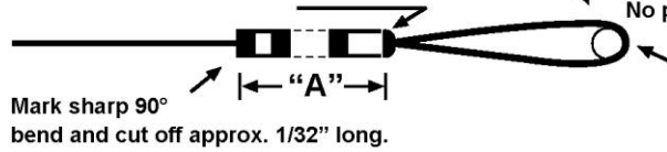
Figure 1A. Two Line Construction For Us With Button-Type Bellcranks. "Double Loop" Termination.
